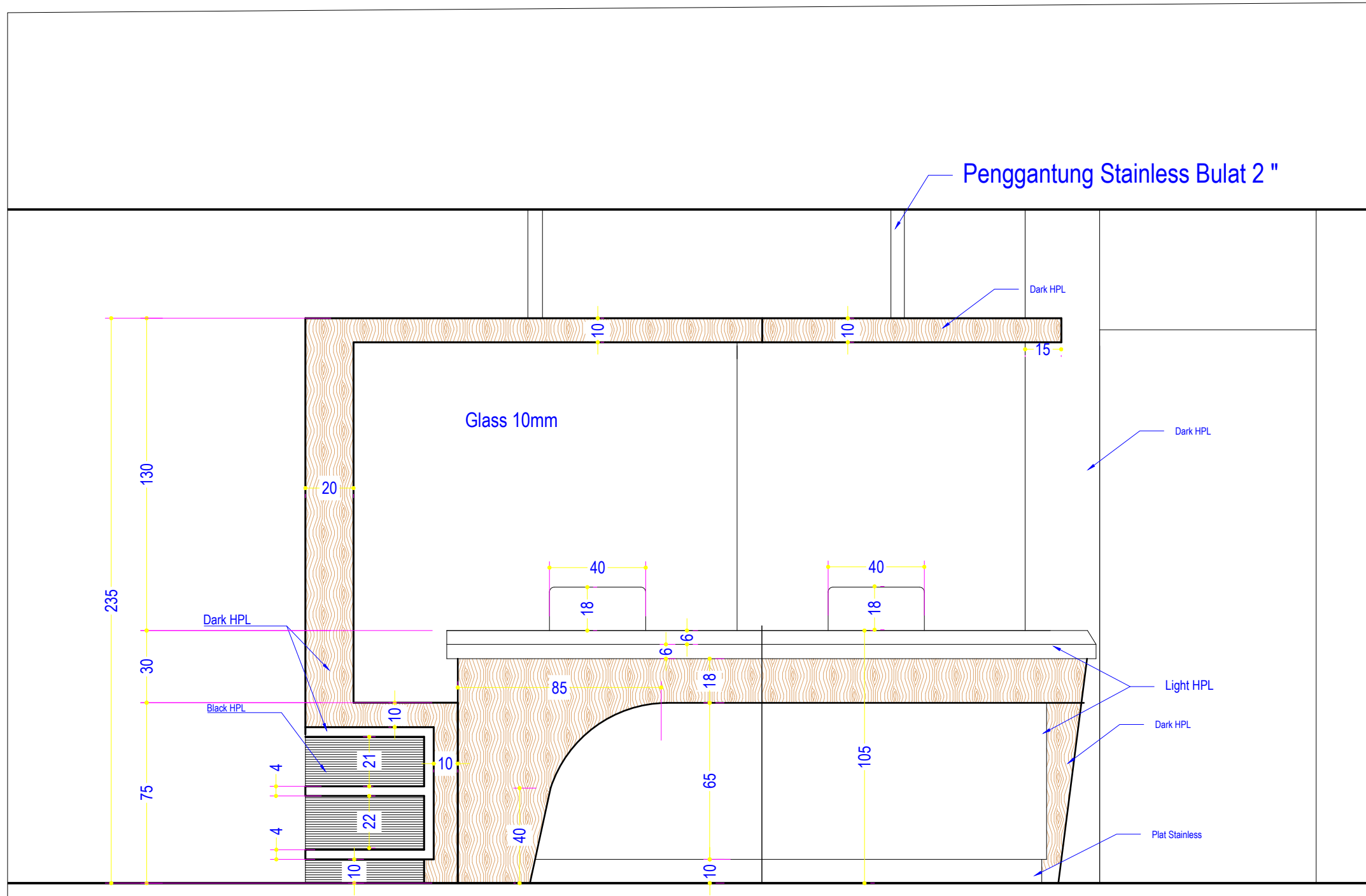
TAMPAK FRONT DESK SKALA 1: 10
