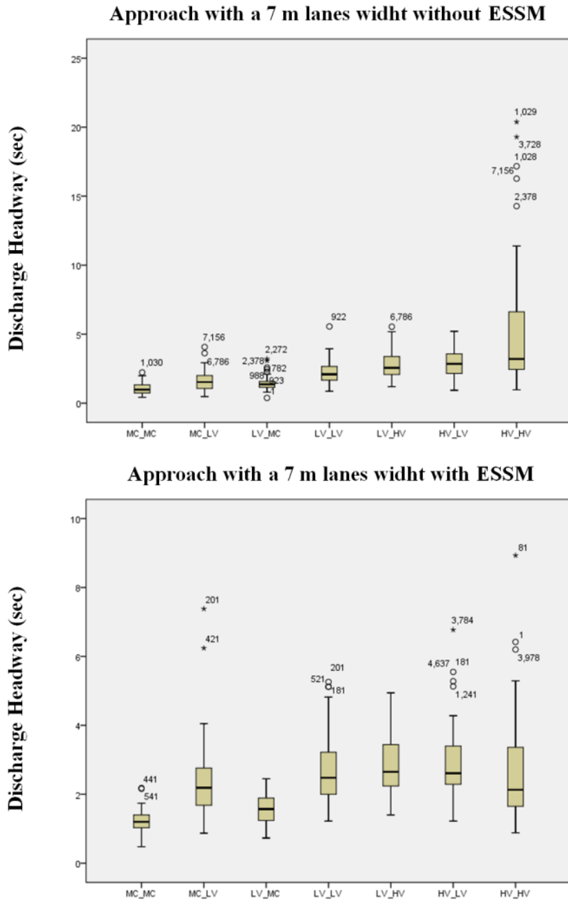
Figure 2. Vehicle Types and Discharge Headways
