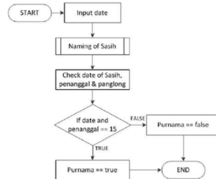
Figure 3. Flowchart of Full Moon Indication
